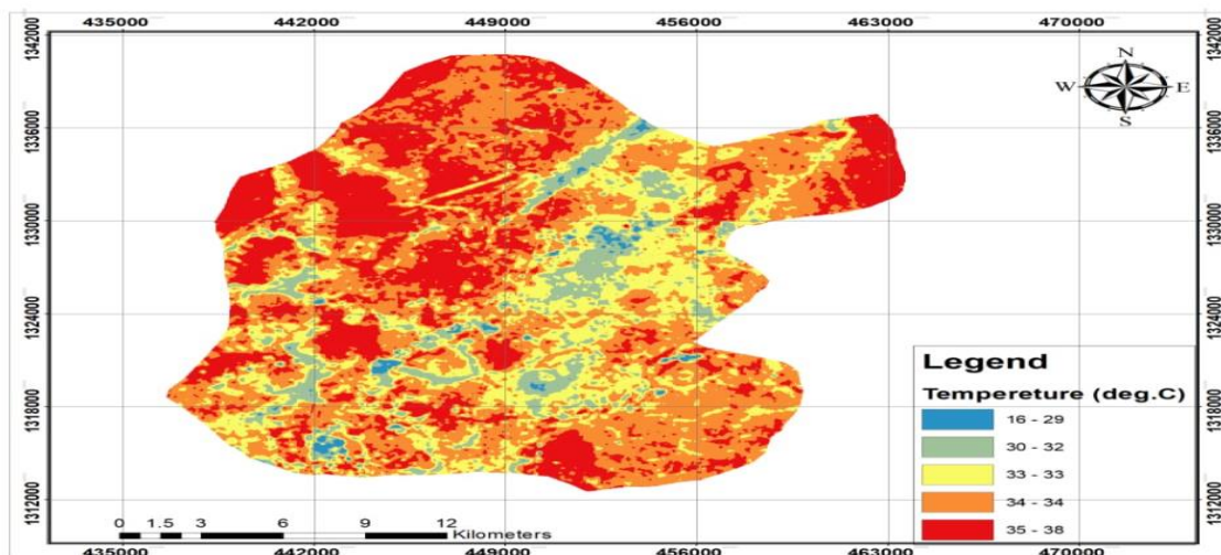
Figure. 2: Estimated Land Surface Temperature From Landsat 5 Thermal Band Information (April 18th, 1991, 18:50:31.896). The Image Spatial Resolution is 120 \times 120 m.
